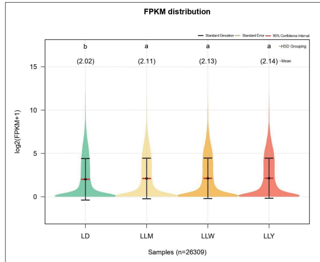
Supplementary Figure 1. Sample comparable quality estimation using the FPKM distribution ( \log_2(\text{FPKM}+1) ), predicted through Tukey's HSD test showing significant difference between control (LD) and treated samples (LLW, LLM, and LLY).
